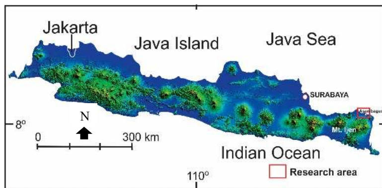
FIGURE 1. Location map of the Asembagus research area.
